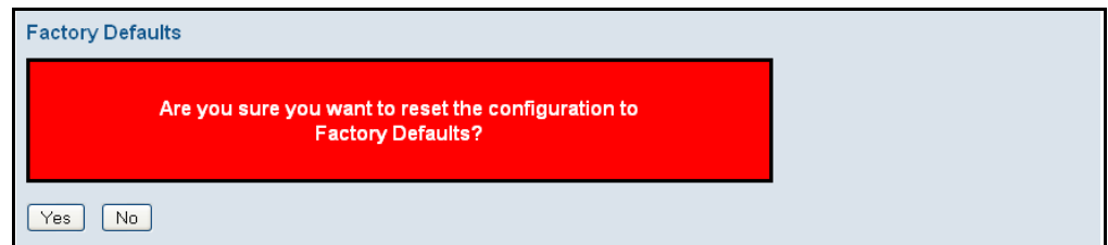
Figure 132: Factory Defaults
