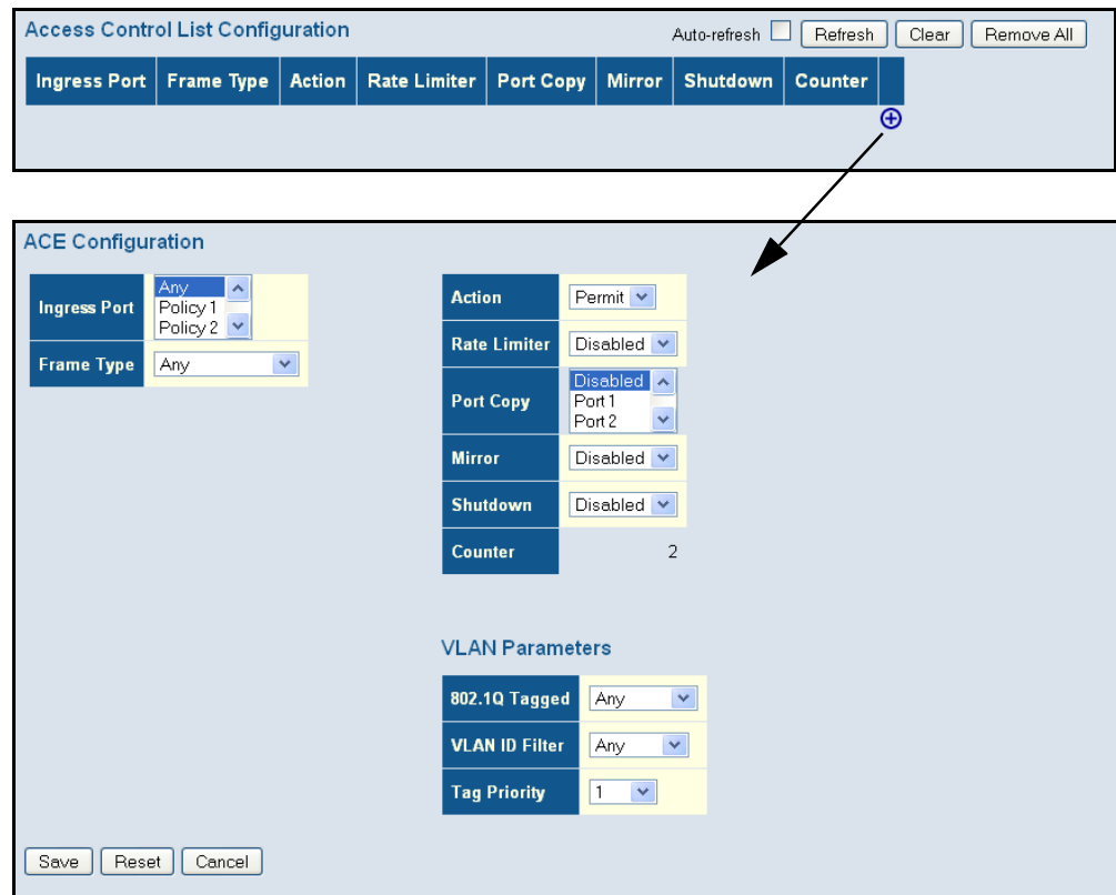
Figure 31: Access Control List Configuration
