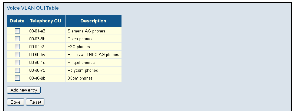
Figure 68: Configuring an OUI Telephony List
