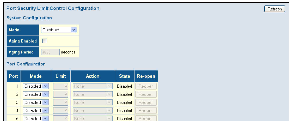
Figure 26: Port Limit Control Configuration
