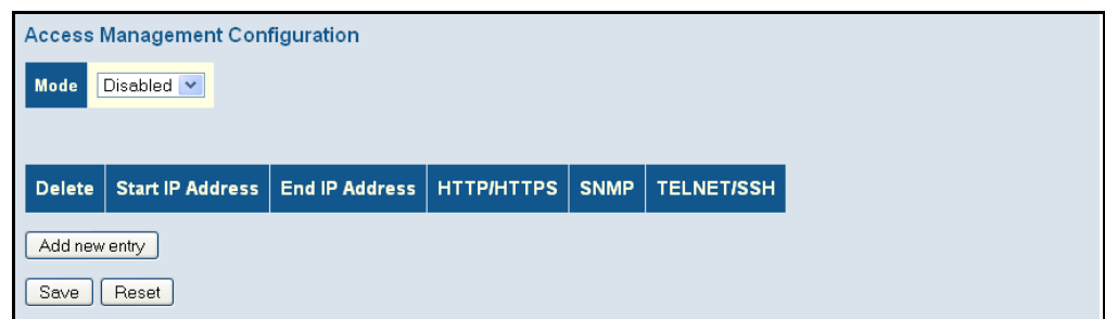
Figure 19: Access Management Configuration
