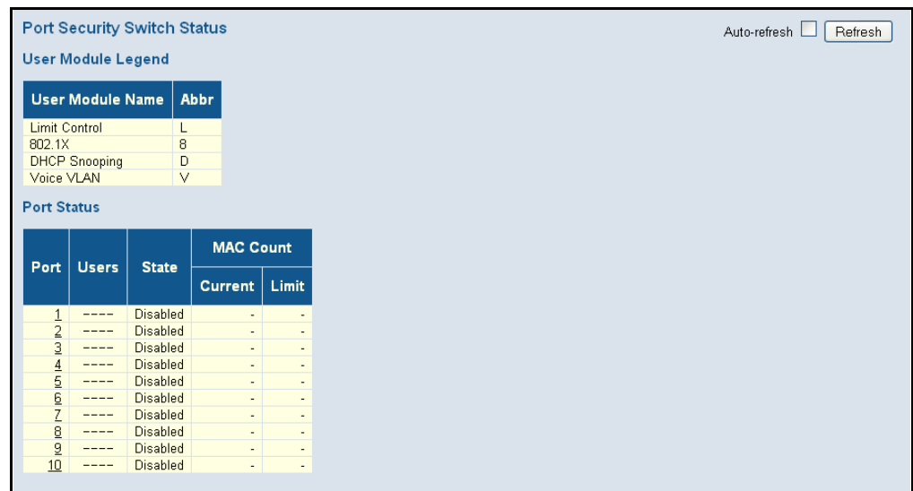
Figure 95: Port Security Switch Status
