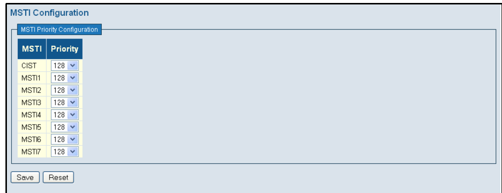
Figure 46: Configuring STA Bridge Priorities
