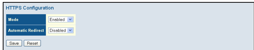
Figure 18: HTTPS Configuration
