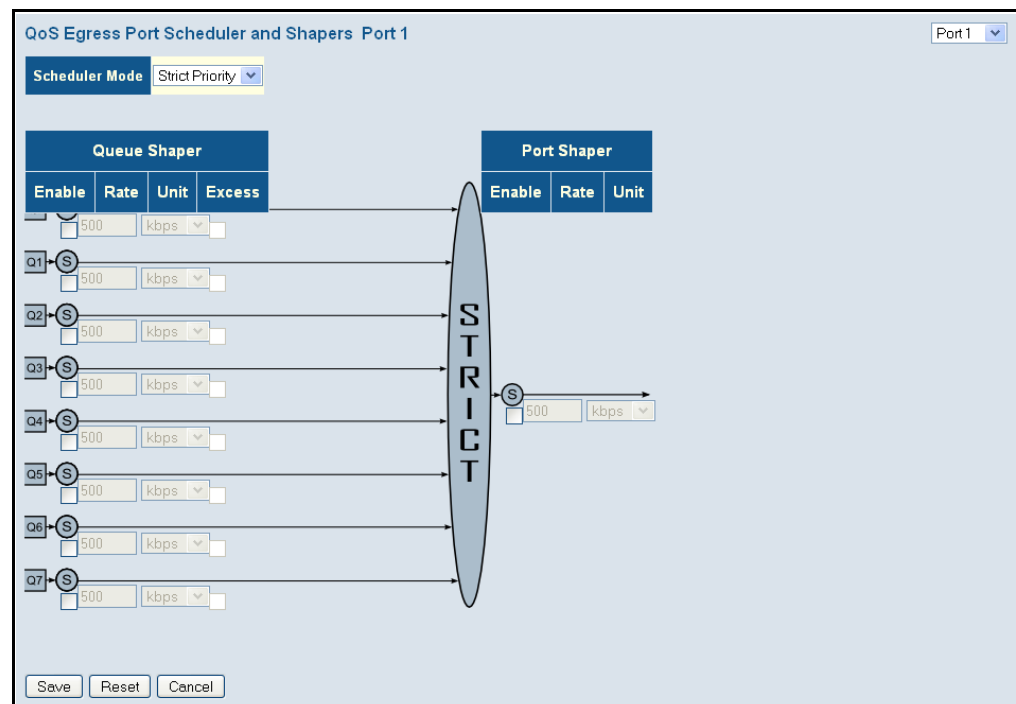
Figure 72: Configuring Egress Port Schedulers and Shapers
