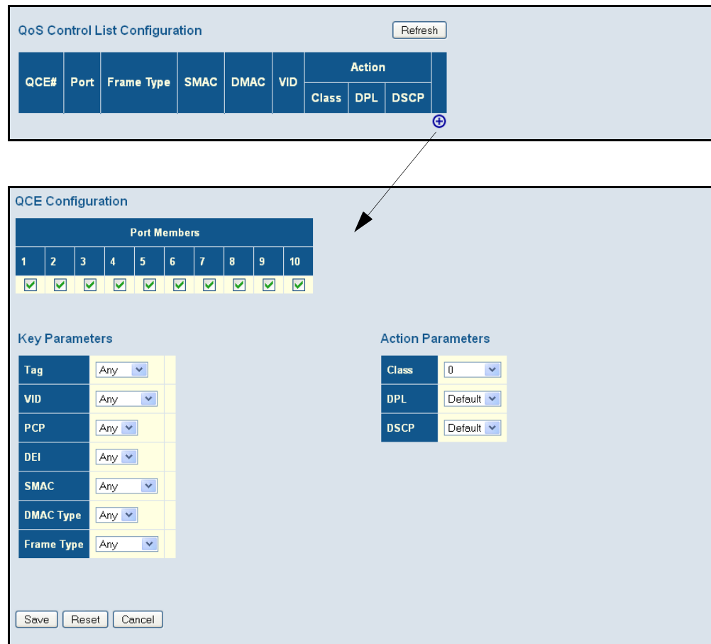
Figure 80: QoS Control List Configuration
