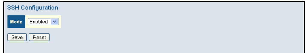
Figure 17: SSH Configuration
